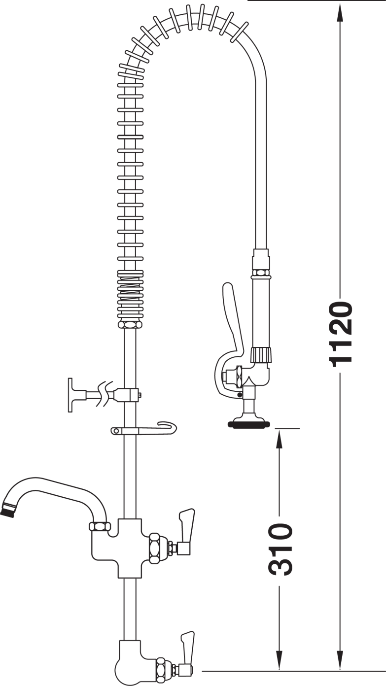
(F) 1/2-inch connection Tap hole req.: 25mm dia.
