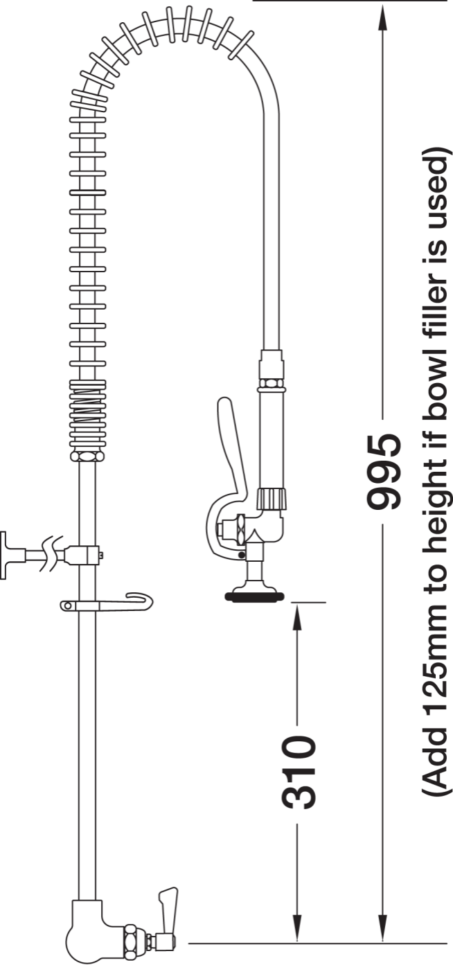
(F) 1/2-inch connection Tap hole req.: 25mm dia.
