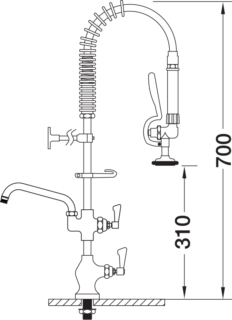
(M) 1/2-inch connection Tap hole req.: 25mm dia.
