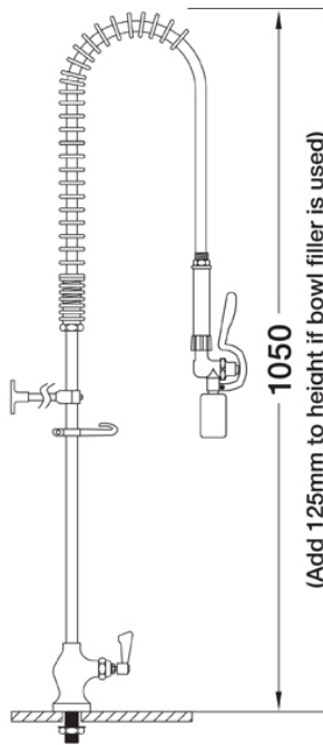
(M) 1/2-inch connection Tap hole req.: 25mm dia.
