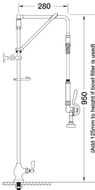
(M) 1/2-inch connection Tap hole req.: 25mm dia.
